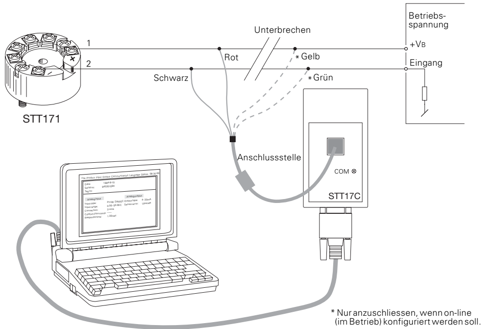
Figure 3-4 Programmierung
