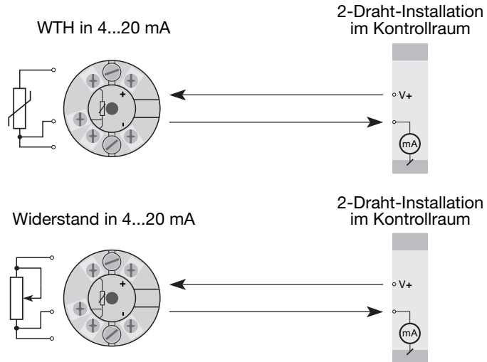
Figure 3-1 2-Draht-Installation
