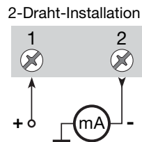
Figure 3-2 Anschlüsse
