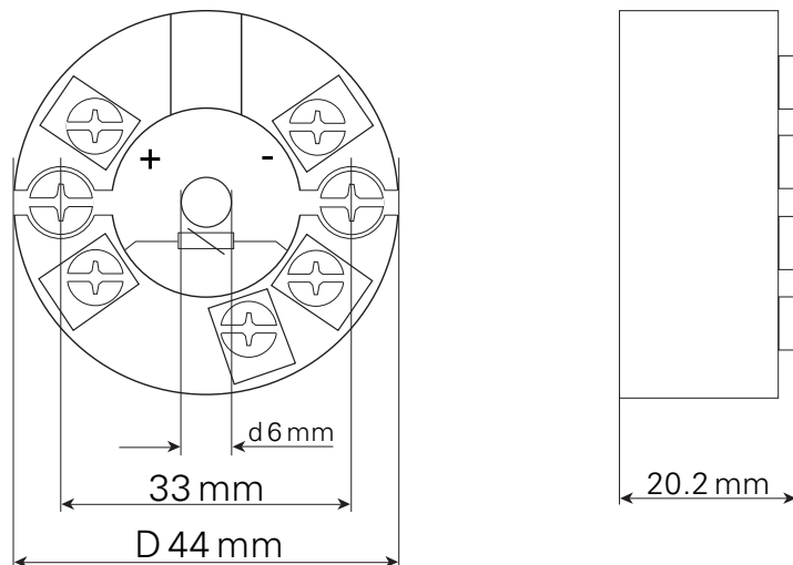
Figure 1-7 Mechanical Specifications
