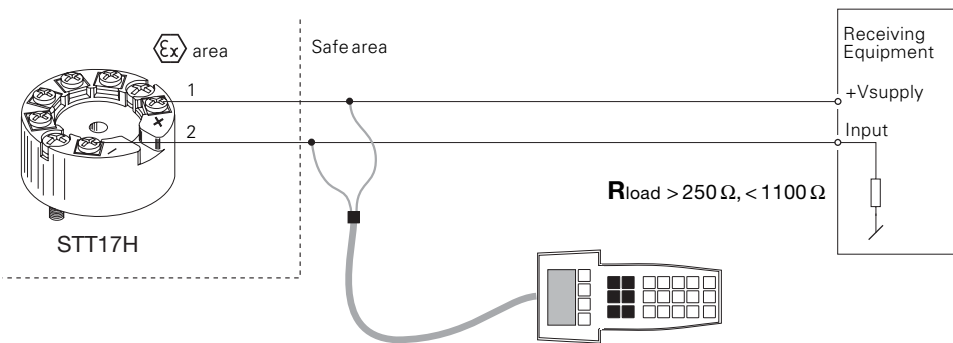
Figure 1-5 HART ® Communicator
