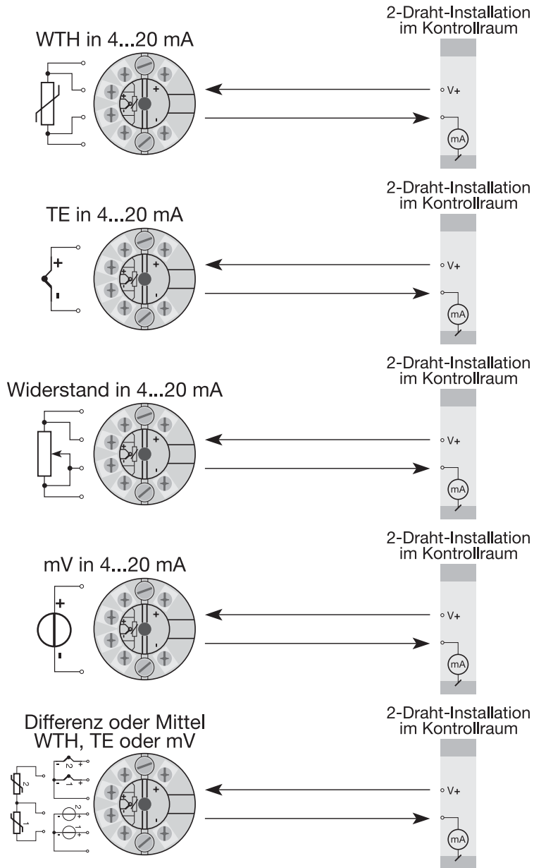
Figure 3-1 2-Draht-Installation
