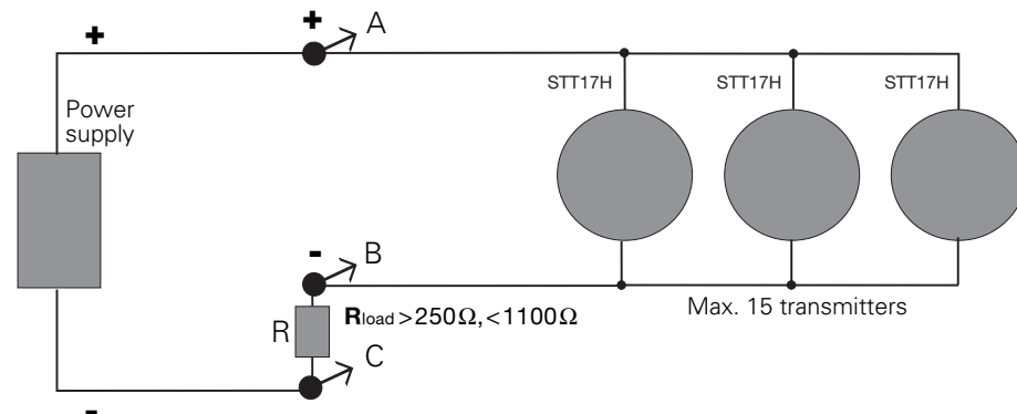
Figure 1-6 Connection of Transmitter in Multi-drop Mode
