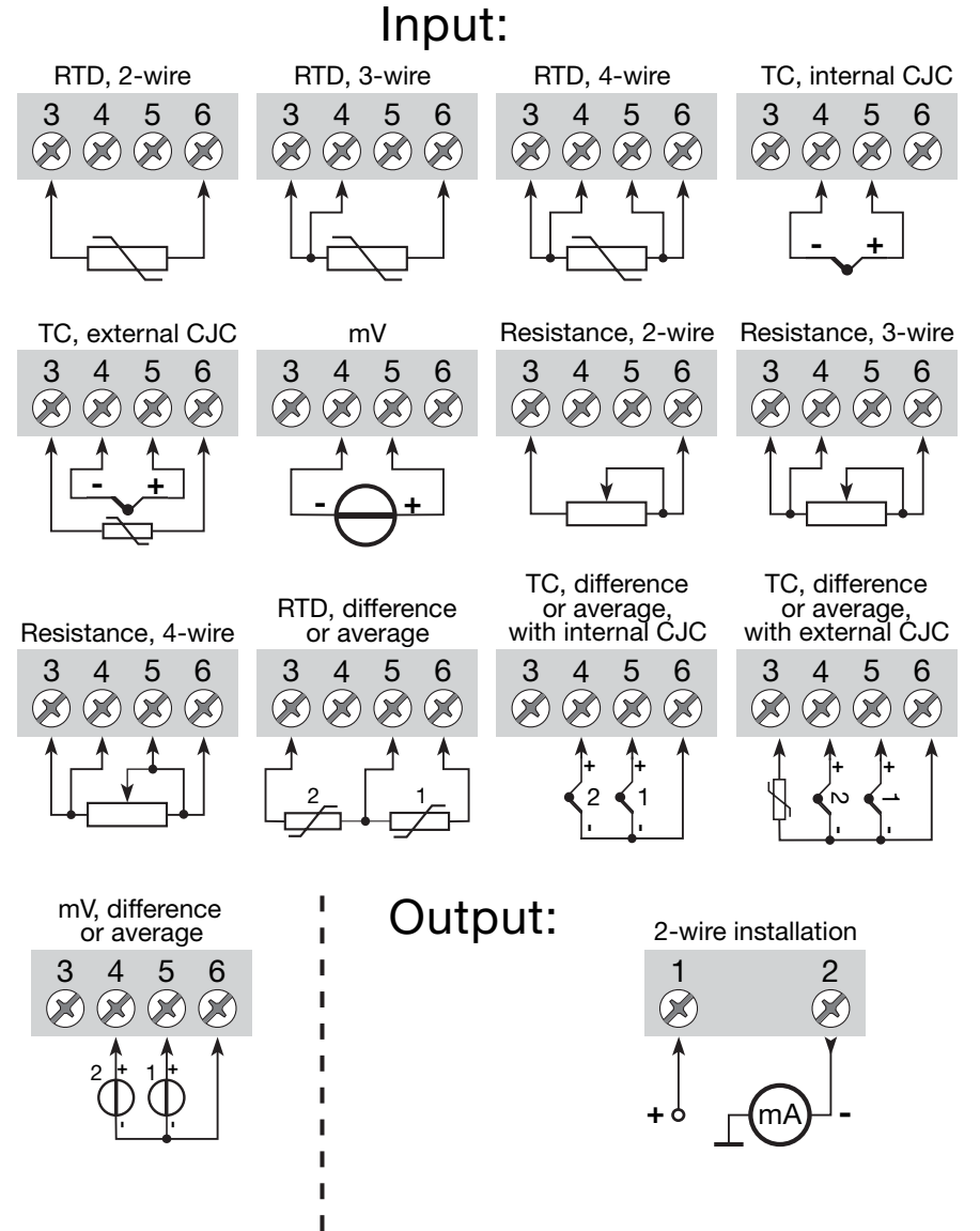
Figure 1-2 Electrical Connections
