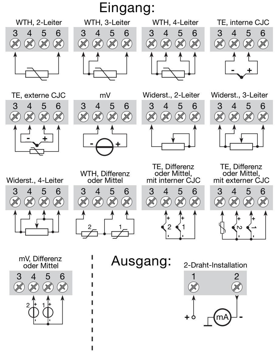
Figure 3-2 Anschlüsse
